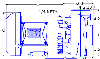
DRAWING DEPICTS 3HP TEFC J56 MOTOR ALL DIMENSIONS IN INCHES
